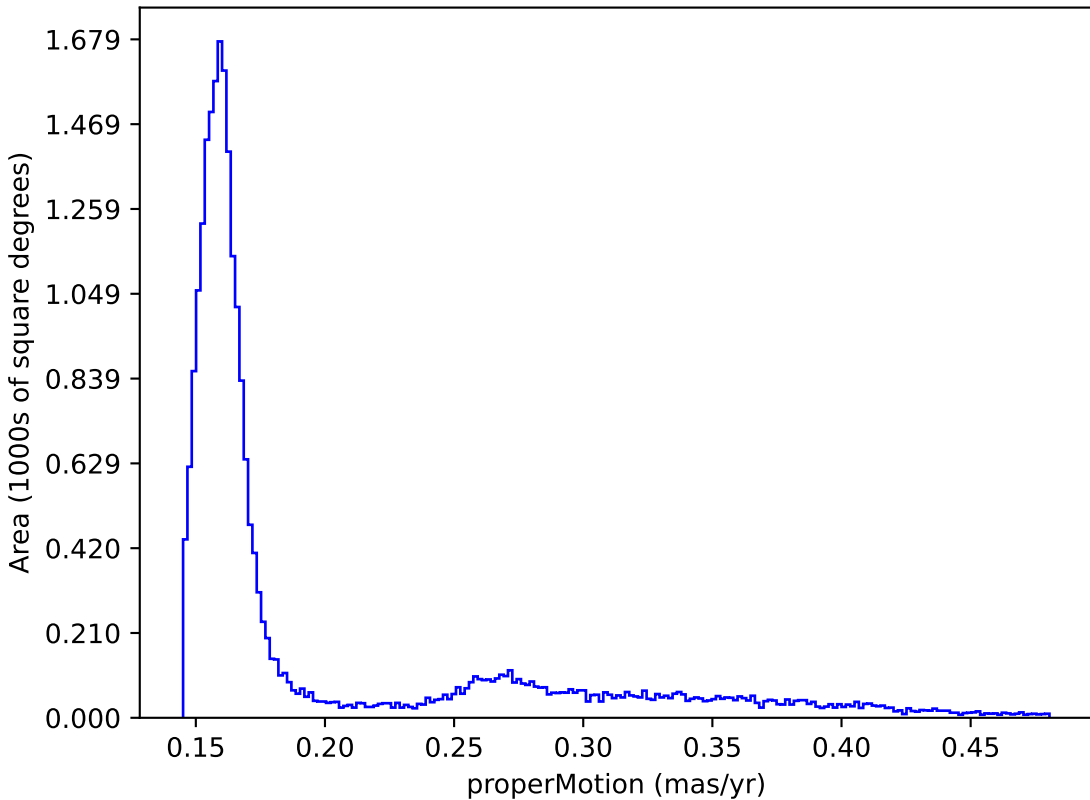
weather_cloudso10v3.5_10yrs : properMotion
