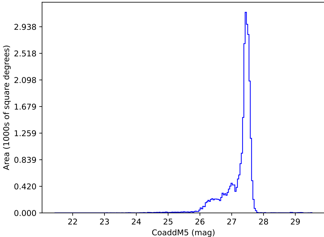
weather_cloudso12v3.5_10yrs : CoaddM5
