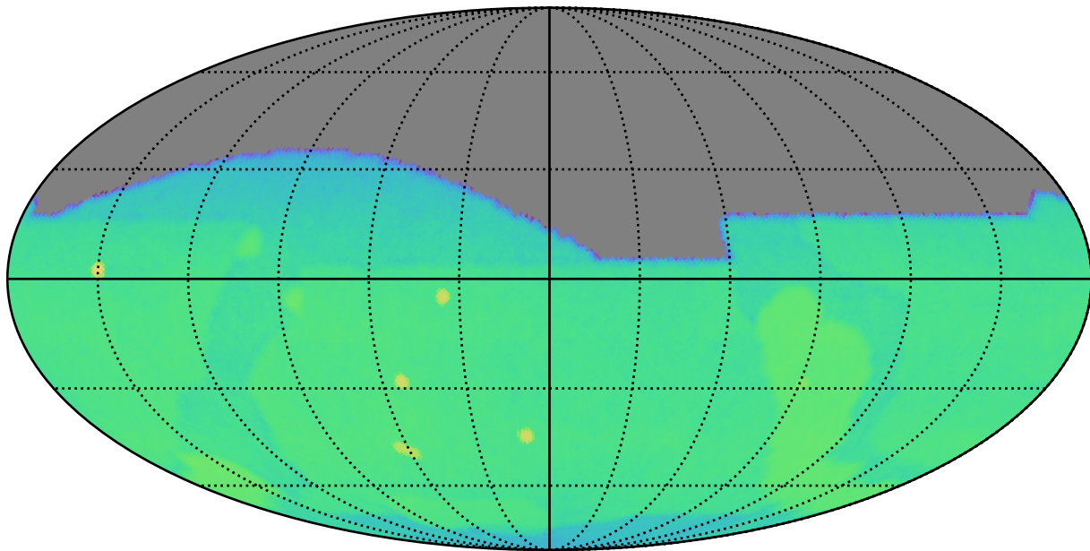
weather_cloudso12v3.5_10yrs g: CoaddM5
