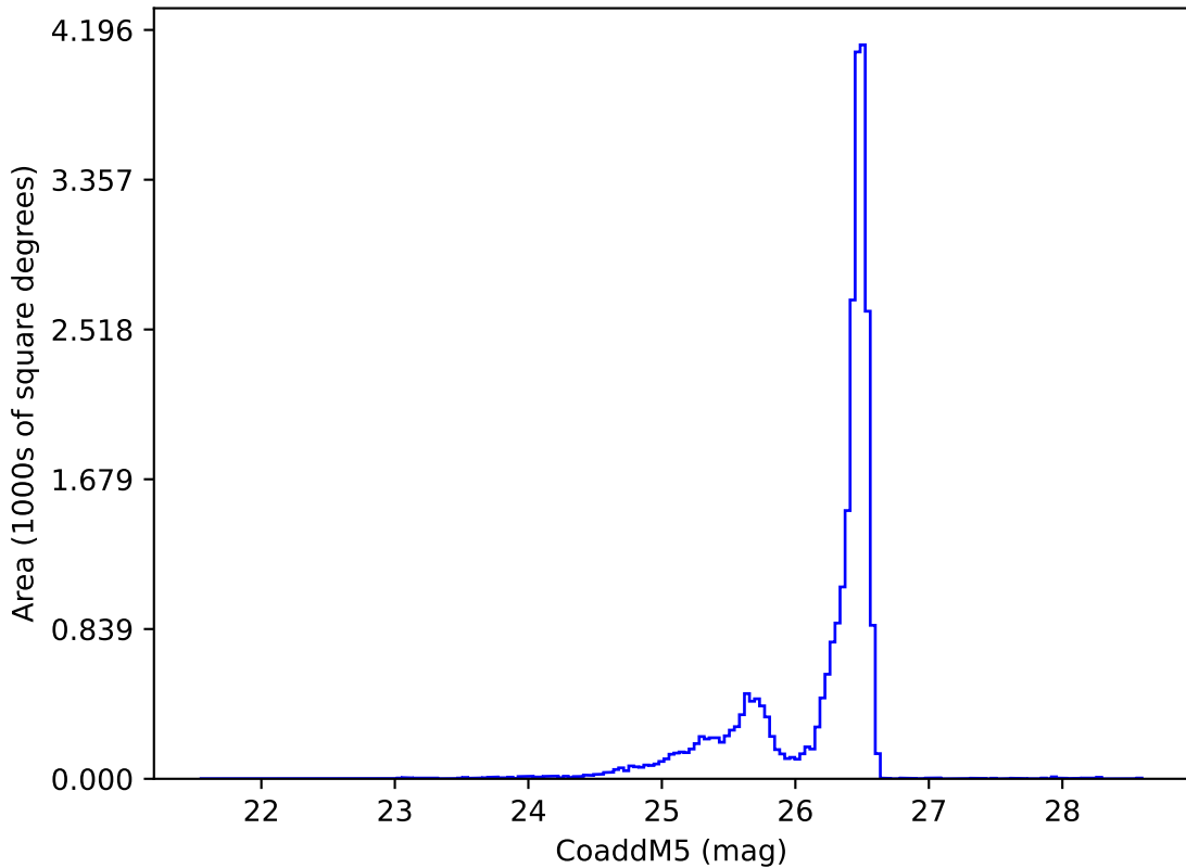
weather_cloudso12v3.5_10yrs i: CoaddM5
