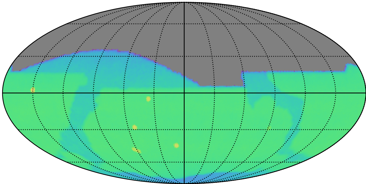
weather_cloudso12v3.5_10yrs i: CoaddM5
