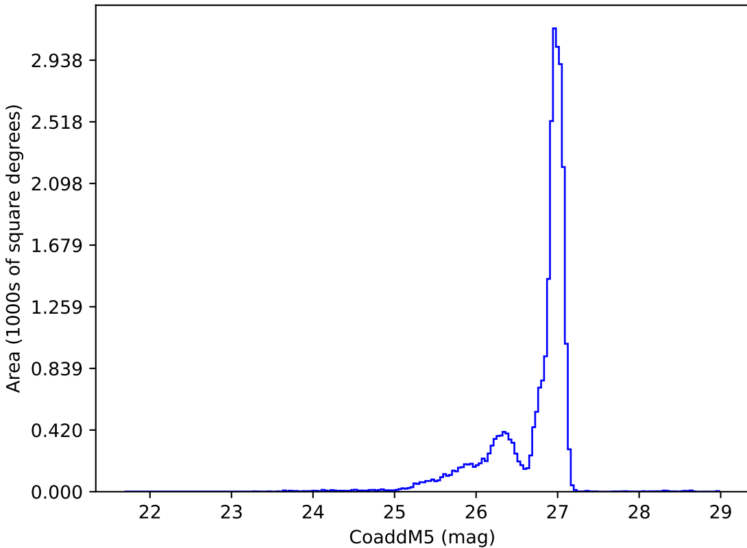
weather_cloudso12v3.5_10yrs r: CoaddM5
