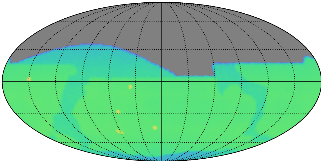
weather_cloudso12v3.5_10yrs r: CoaddM5
