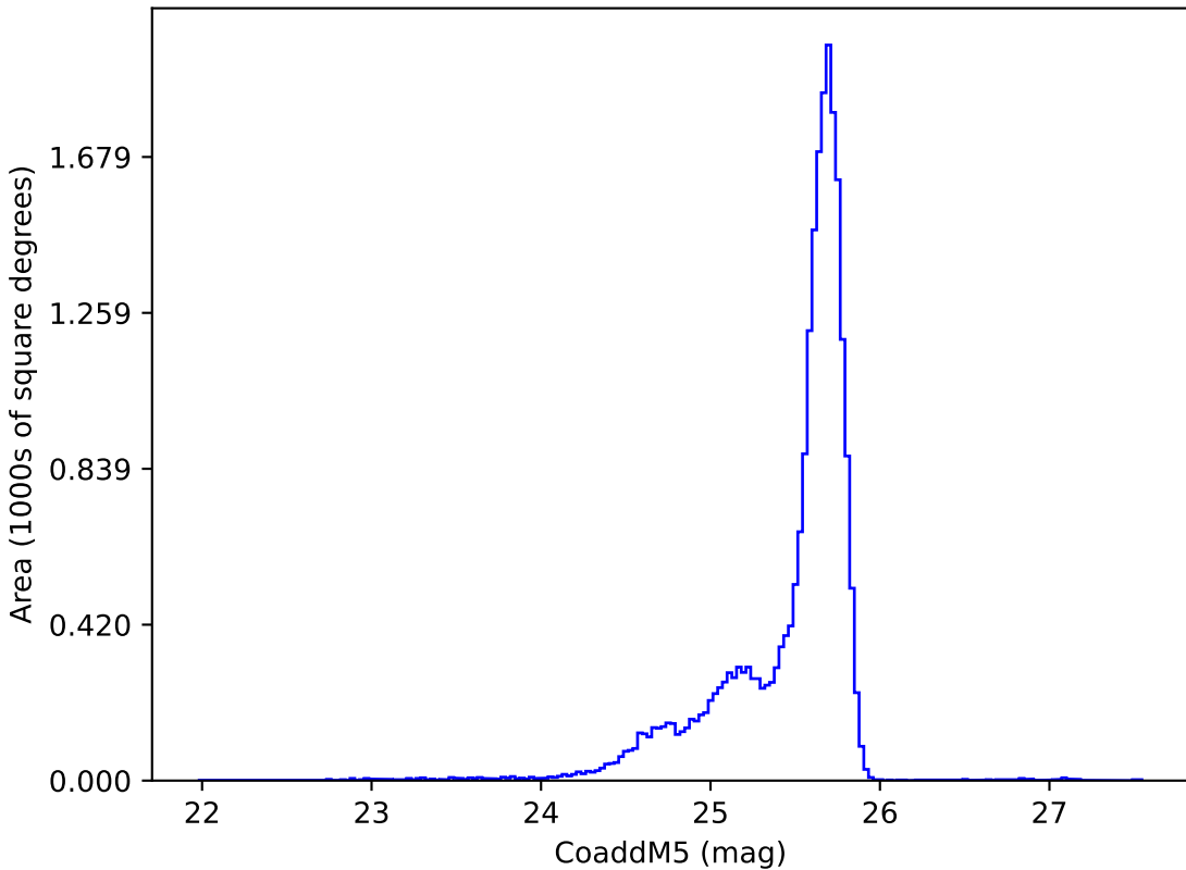
weather_cloudso12v3.5_10yrs u: CoaddM5
