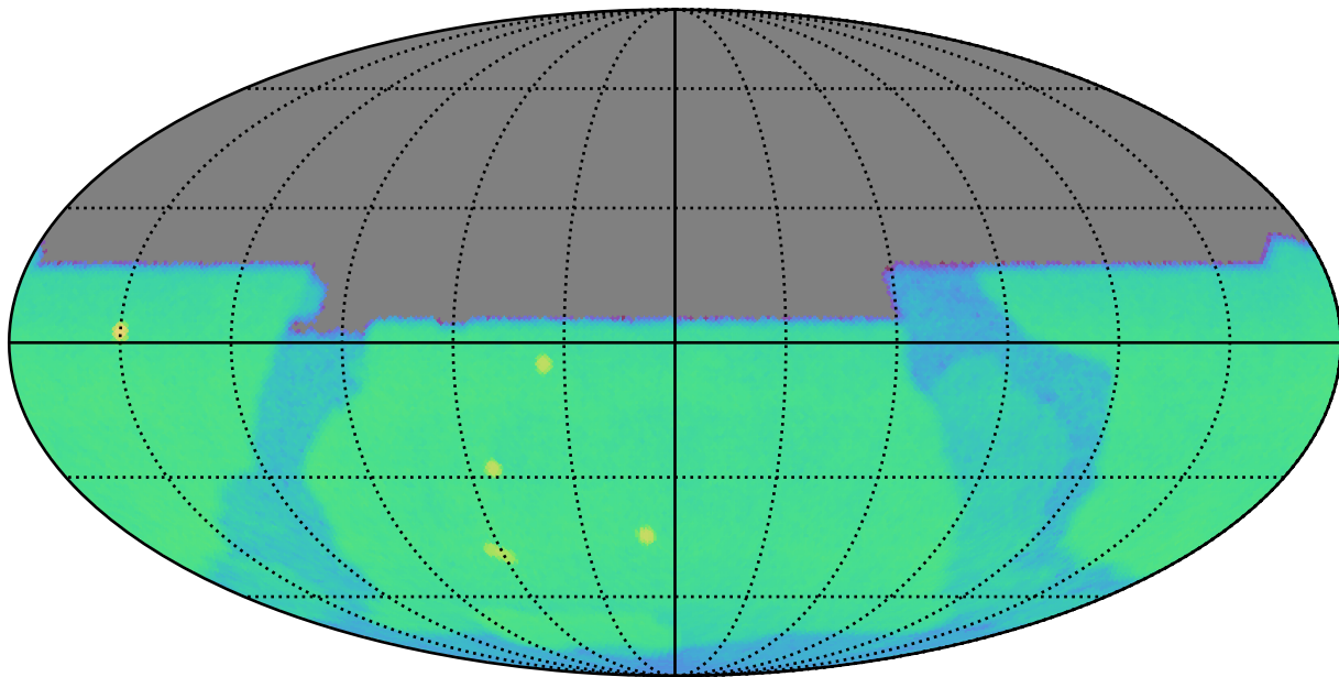
weather_cloudso12v3.5_10yrs u: CoaddM5
