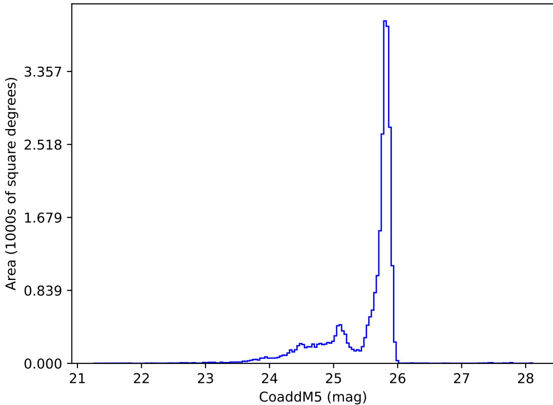
weather_cloudso12v3.5_10yrs z: CoaddM5
