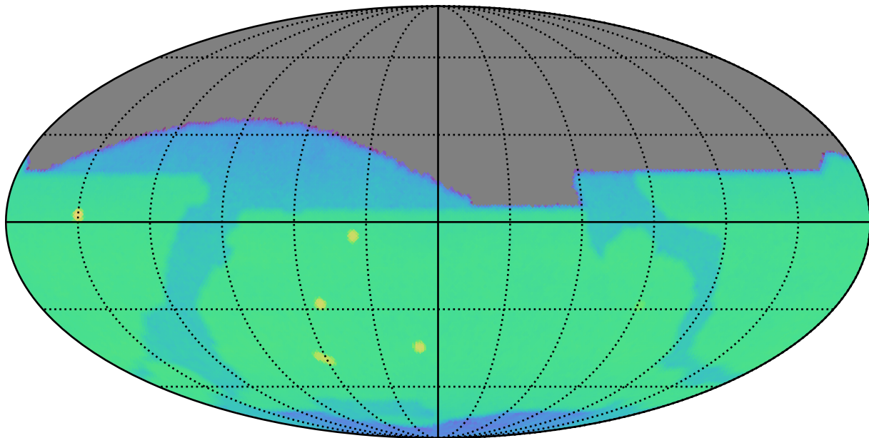
weather_cloudso12v3.5_10yrs z: CoaddM5
