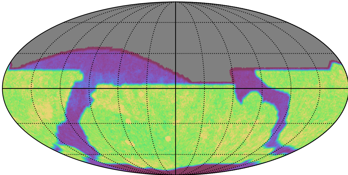
weather_cloudso12v3.5_10yrs r: Count observationStartMJD
