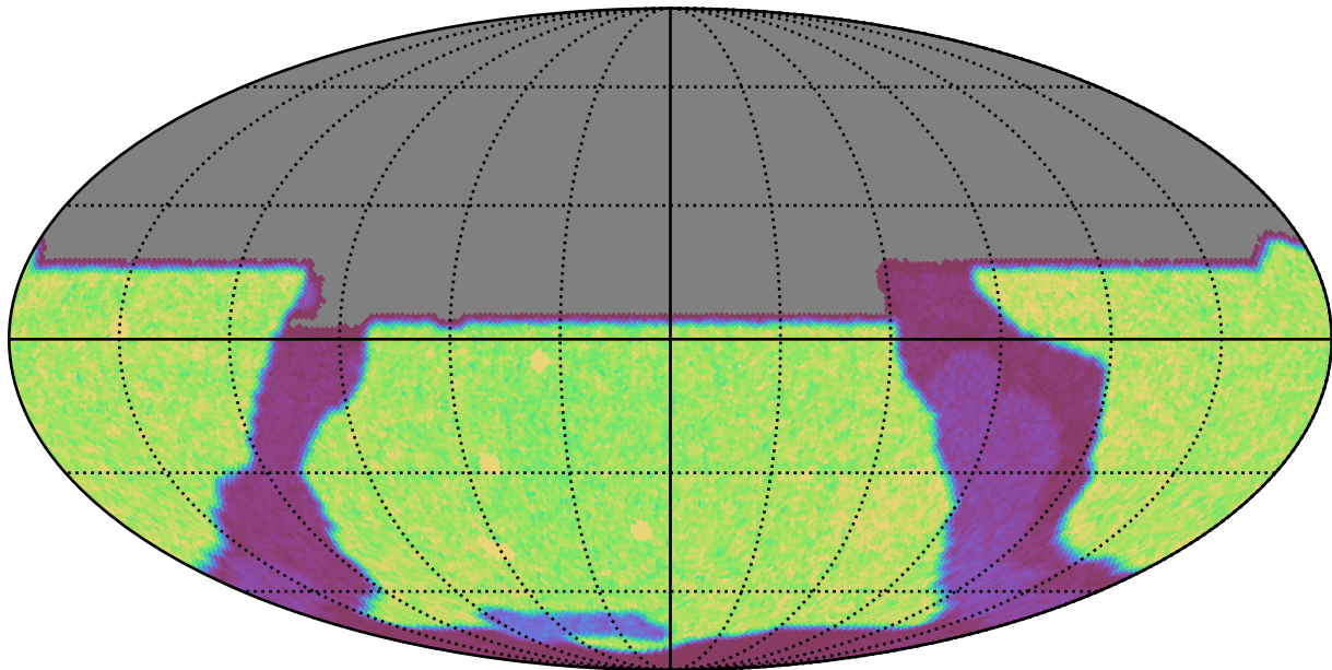
weather_cloudso12v3.5_10yrs y: Count observationStartMJD
