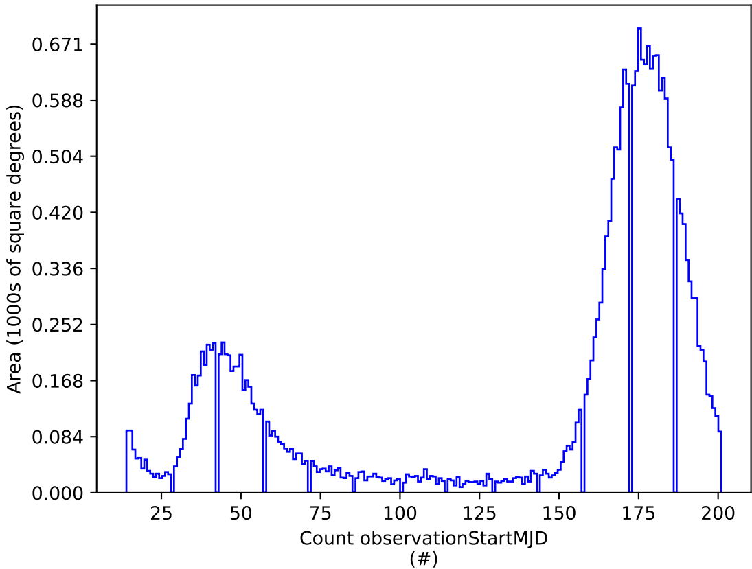
weather_cloudso12v3.5_10yrs z: Count observationStartMJD
