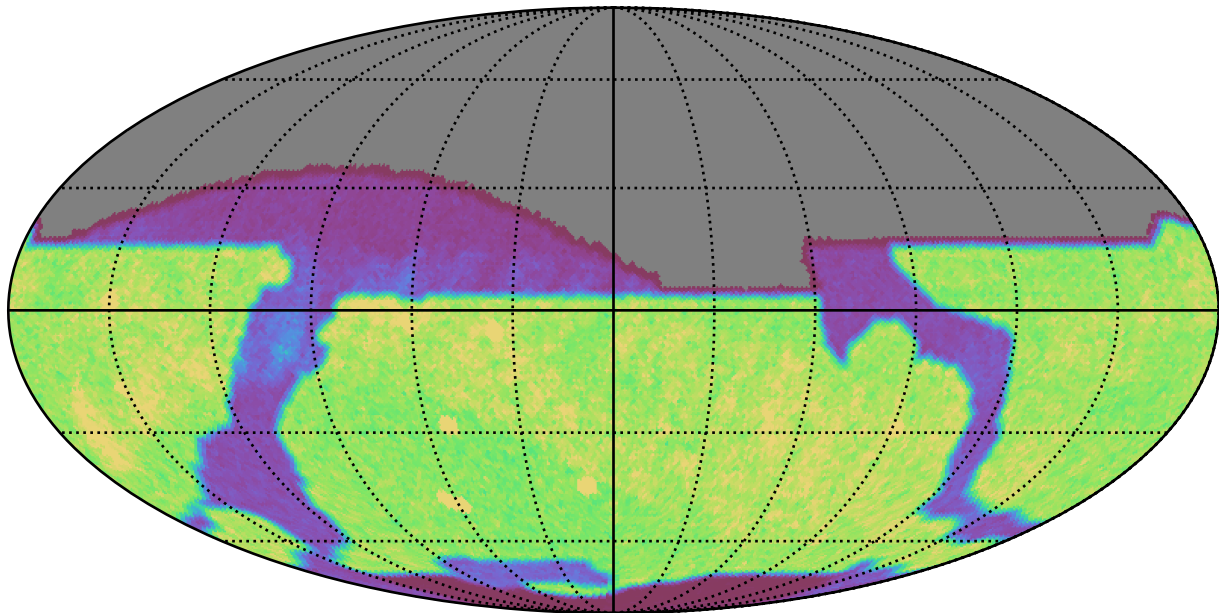
weather_cloudso12v3.5_10yrs z: Count observationStartMJD
