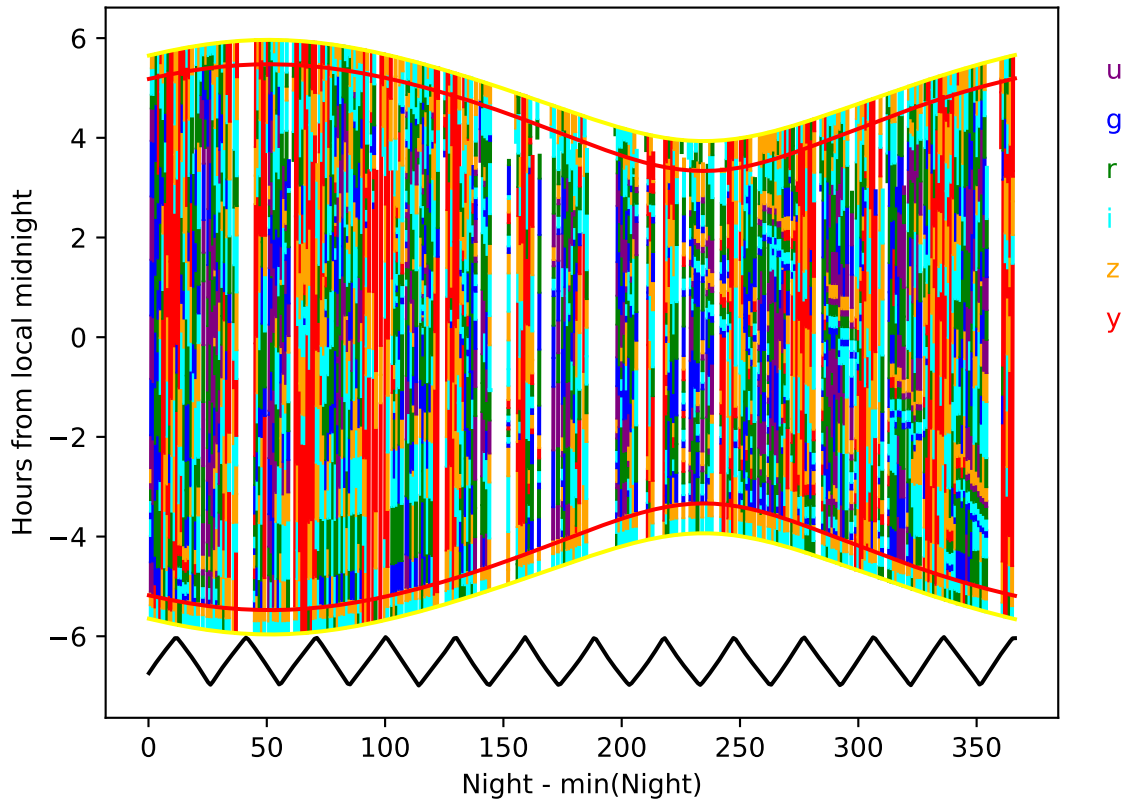
weather_cloudso12v3.5_10yrs year 0-1: Hourglass
