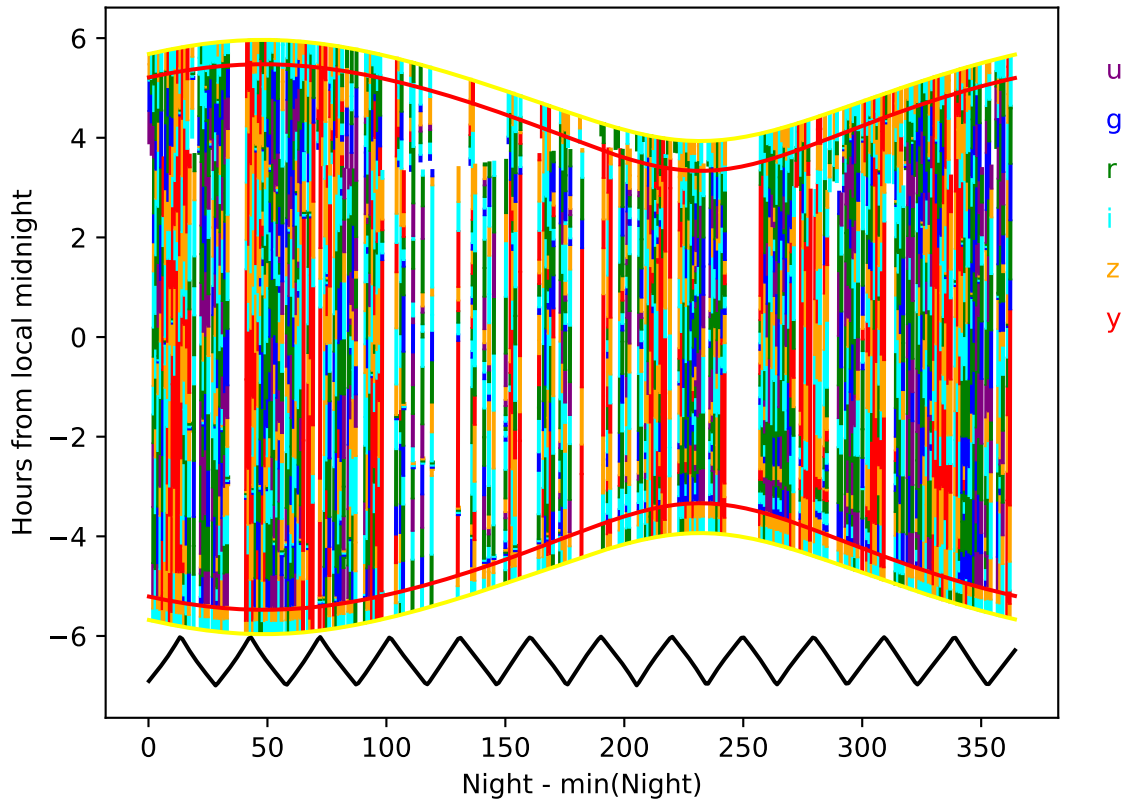
weather_cloudso12v3.5_10yrs year 5-6: Hourglass
