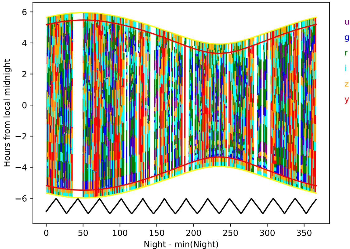
weather_cloudso12v3.5_10yrs year 8-9: Hourglass
