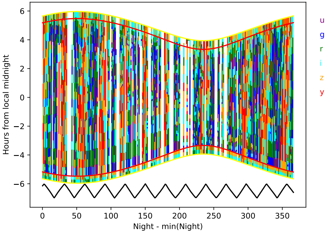
weather_cloudso12v3.5_10yrs year 9-10: Hourglass
