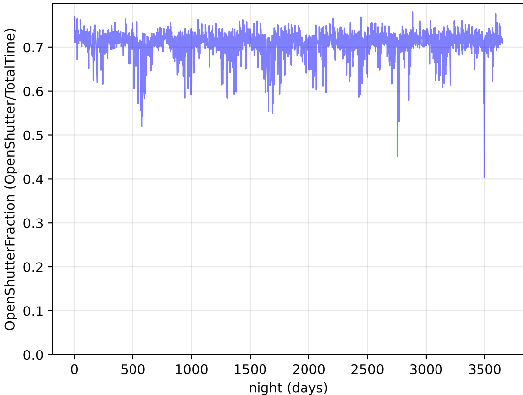
weather_cloudso12v3.5_10yrs : OpenShutterFraction
