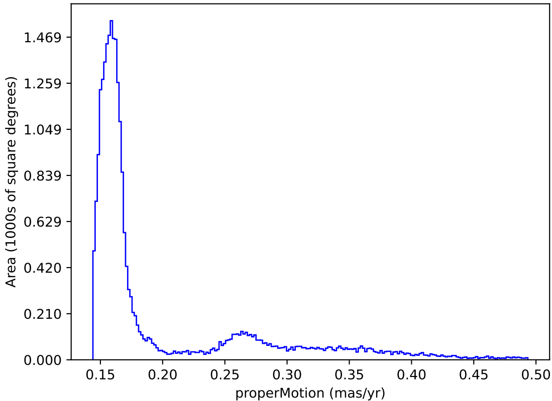
weather_cloudso12v3.5_10yrs : properMotion
