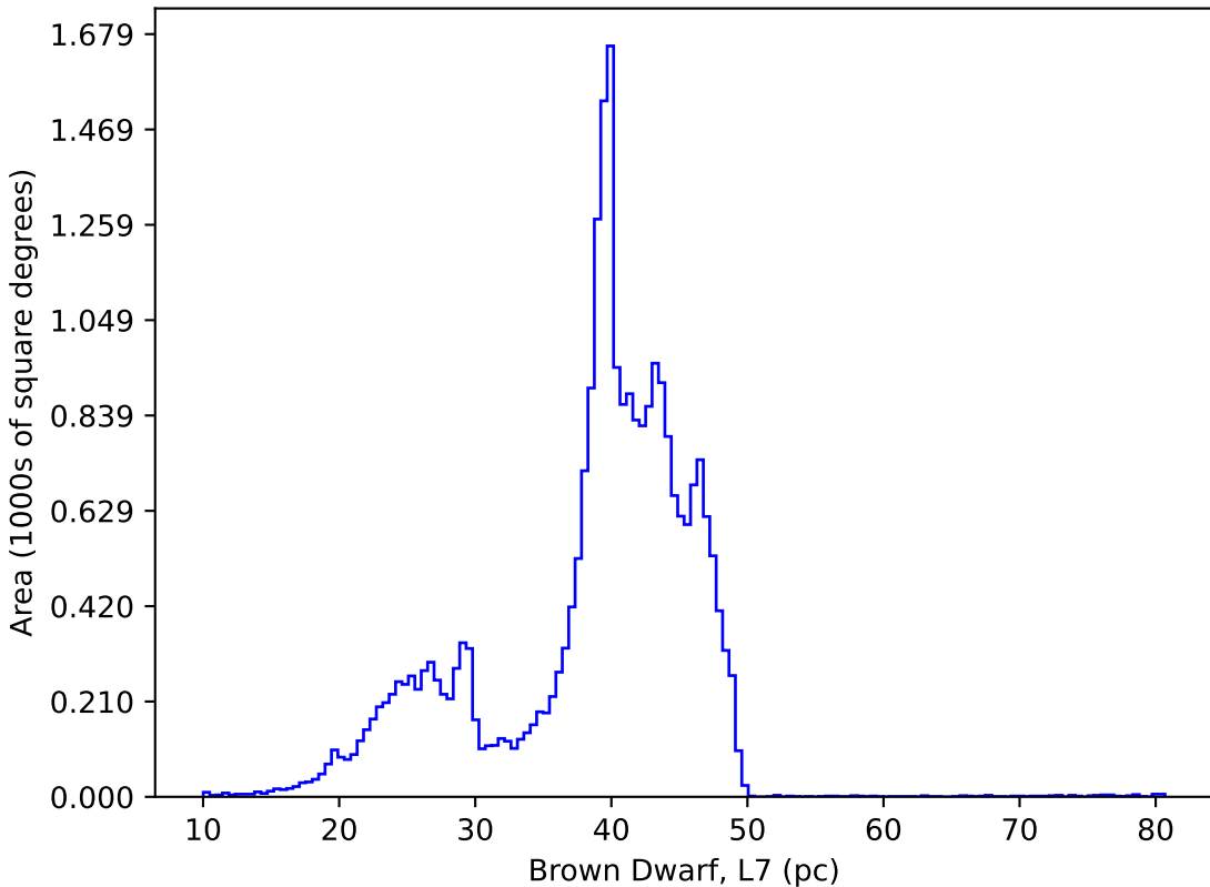
weather_cloudso12v3.5_10yrs : Brown Dwarf, L7
