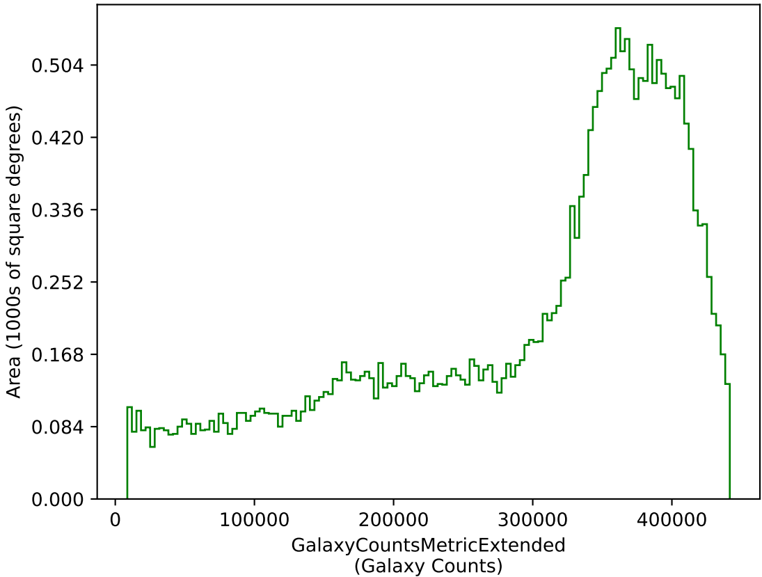
weather_cloudso12v3.5_10yrs g: GalaxyCountsMetricExtended
