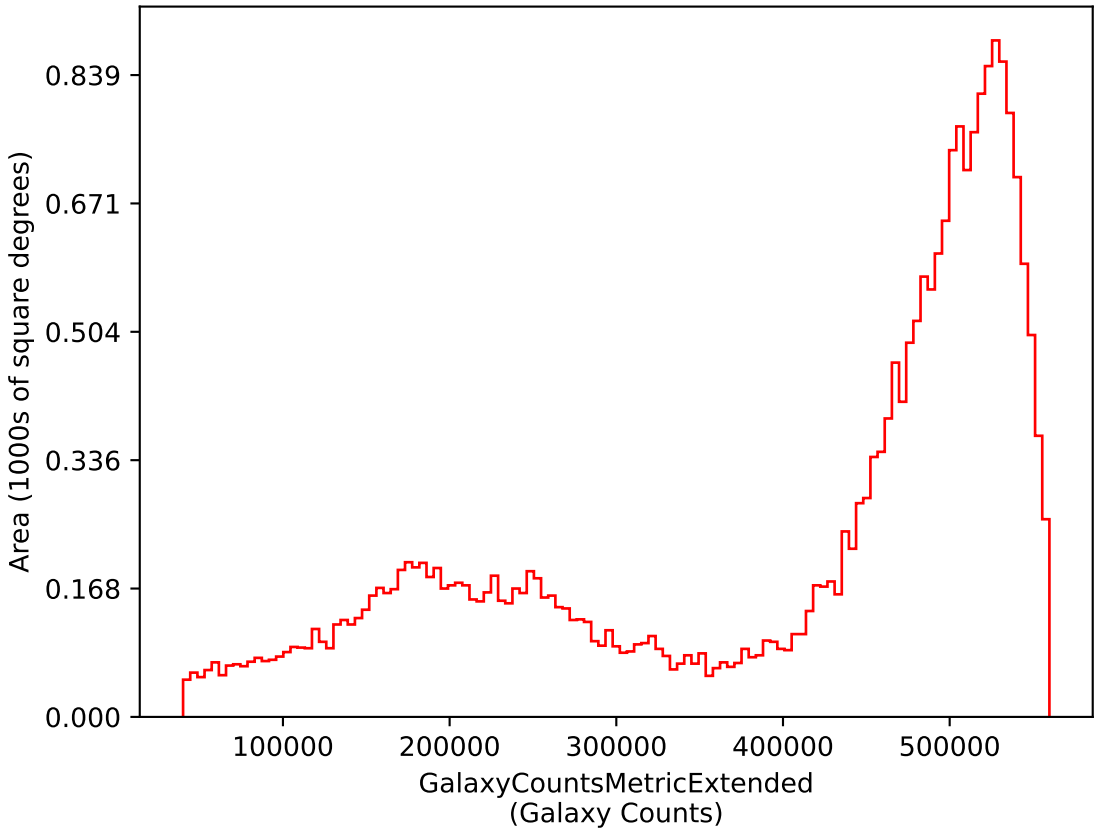
weather_cloudso12v3.5_10yrs i: GalaxyCountsMetricExtended
