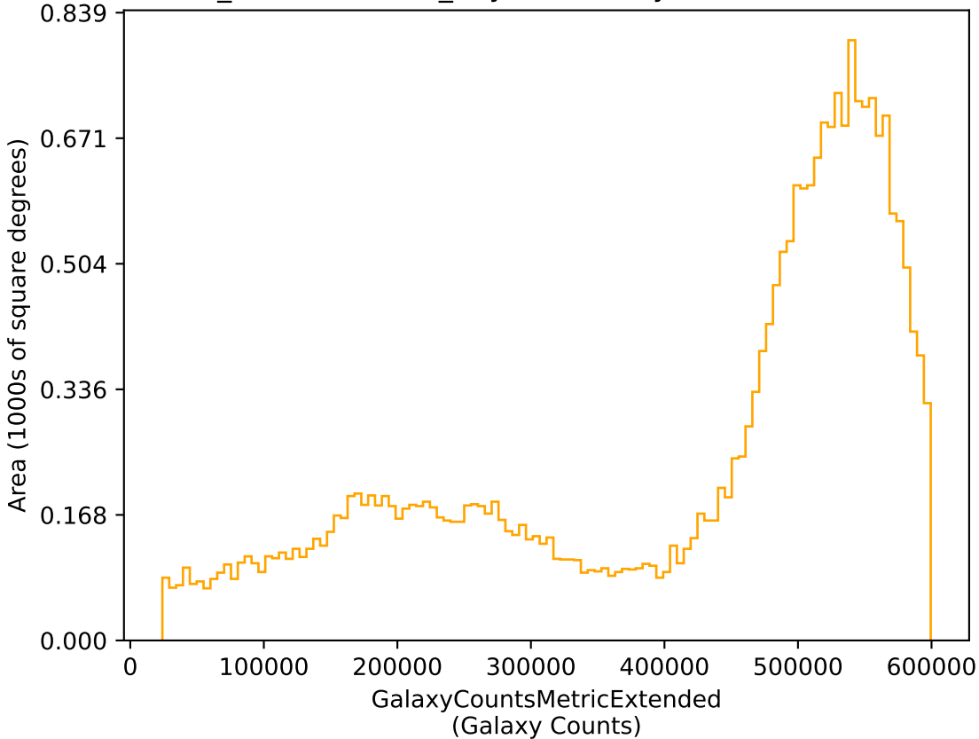
weather_cloudso12v3.5_10yrs r: GalaxyCountsMetricExtended
