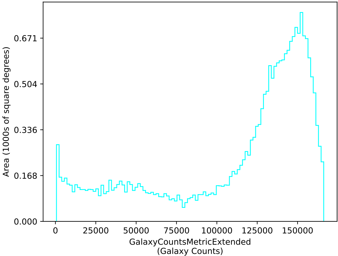
weather_cloudso12v3.5_10yrs u: GalaxyCountsMetricExtended
