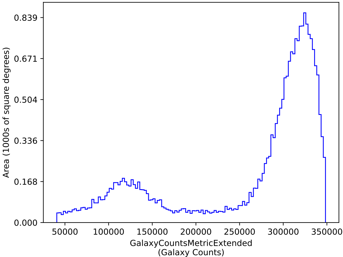
weather_cloudso12v3.5_10yrs y: GalaxyCountsMetricExtended
