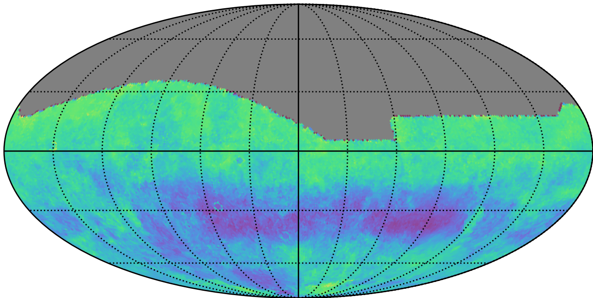
weather_cloudso12v3.5_10yrs g: Kuiper rotSkyPos
