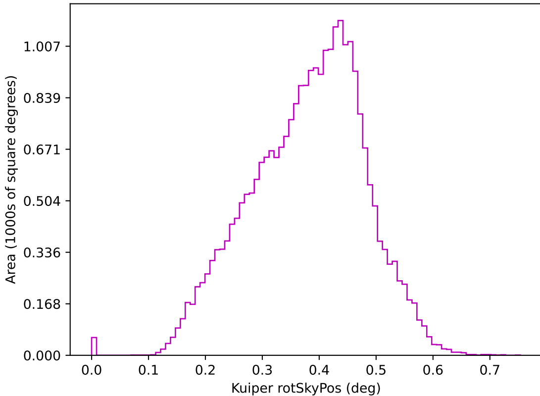
weather_cloudso12v3.5_10yrs z: Kuiper rotSkyPos
