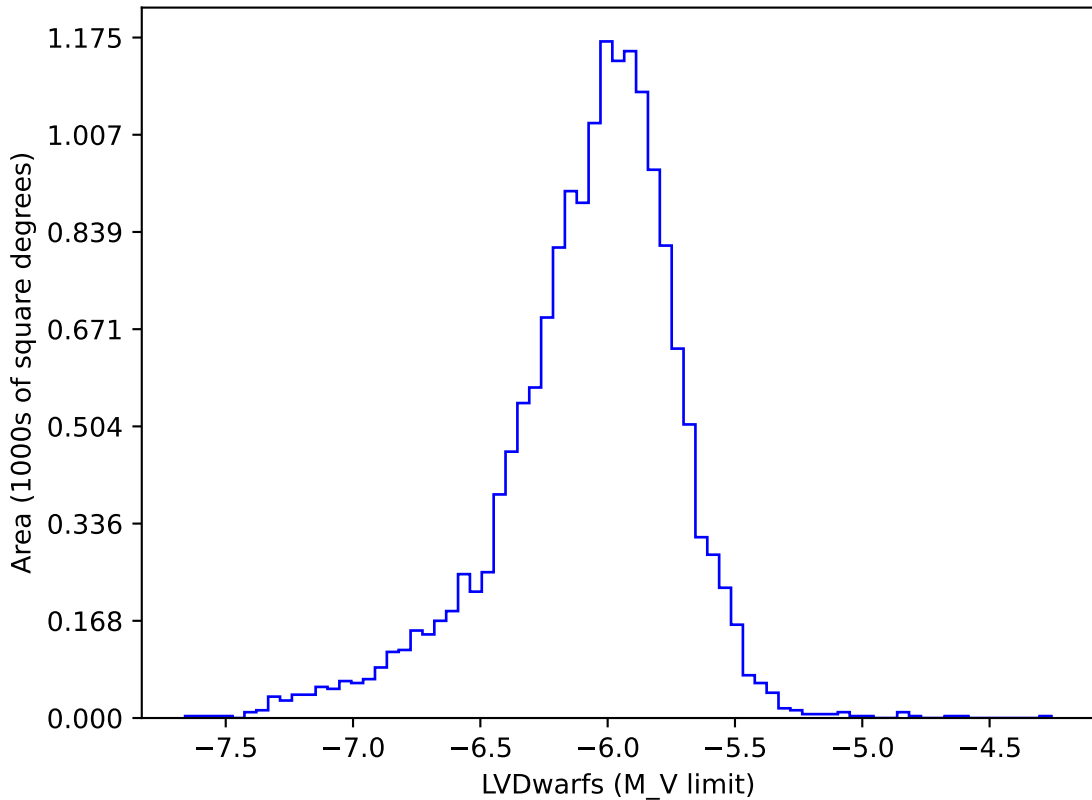
weather_cloudso12v3.5_10yrs gi: LVDwarfs
