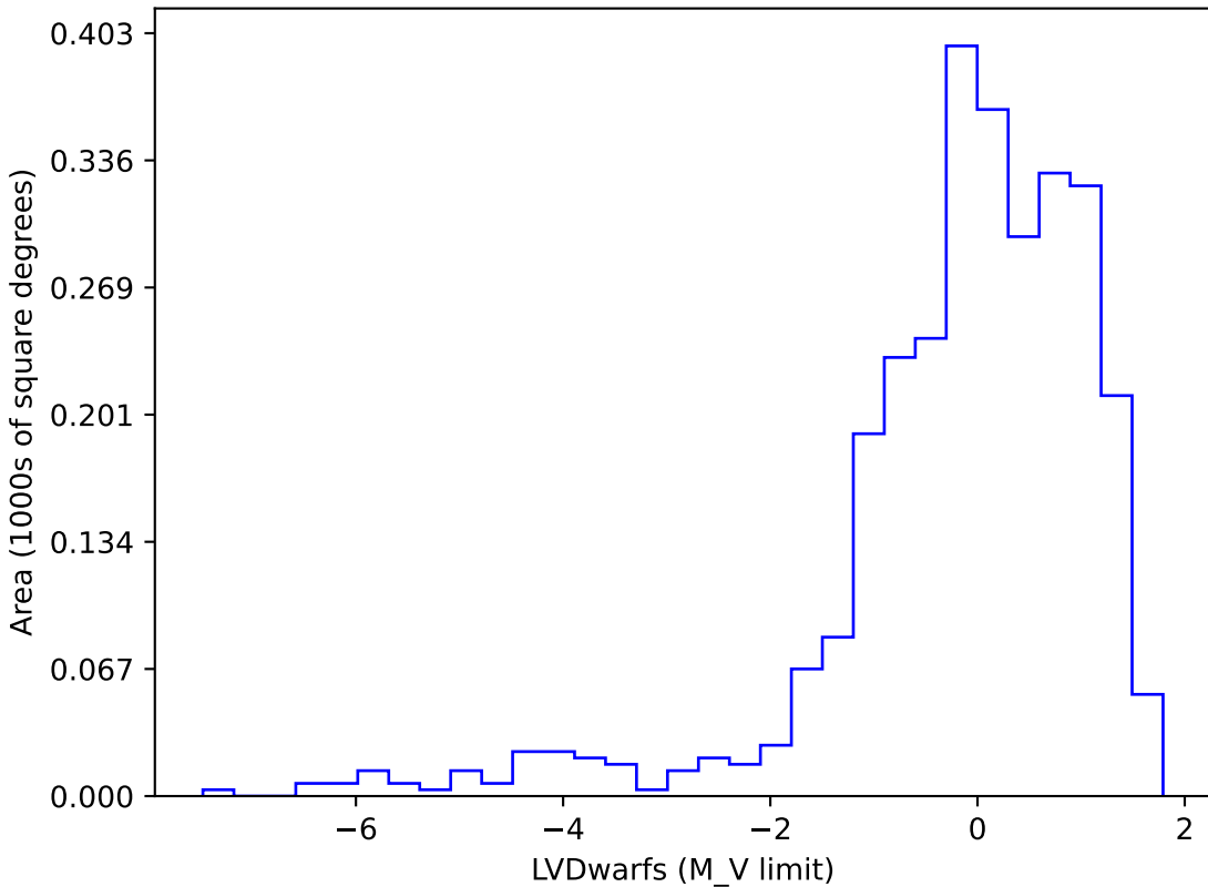
weather_cloudso12v3.5_10yrs gi SCP: LVDwarfs
