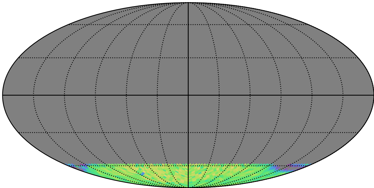
weather_cloudso12v3.5_10yrs gi SCP: LVDwarfs
