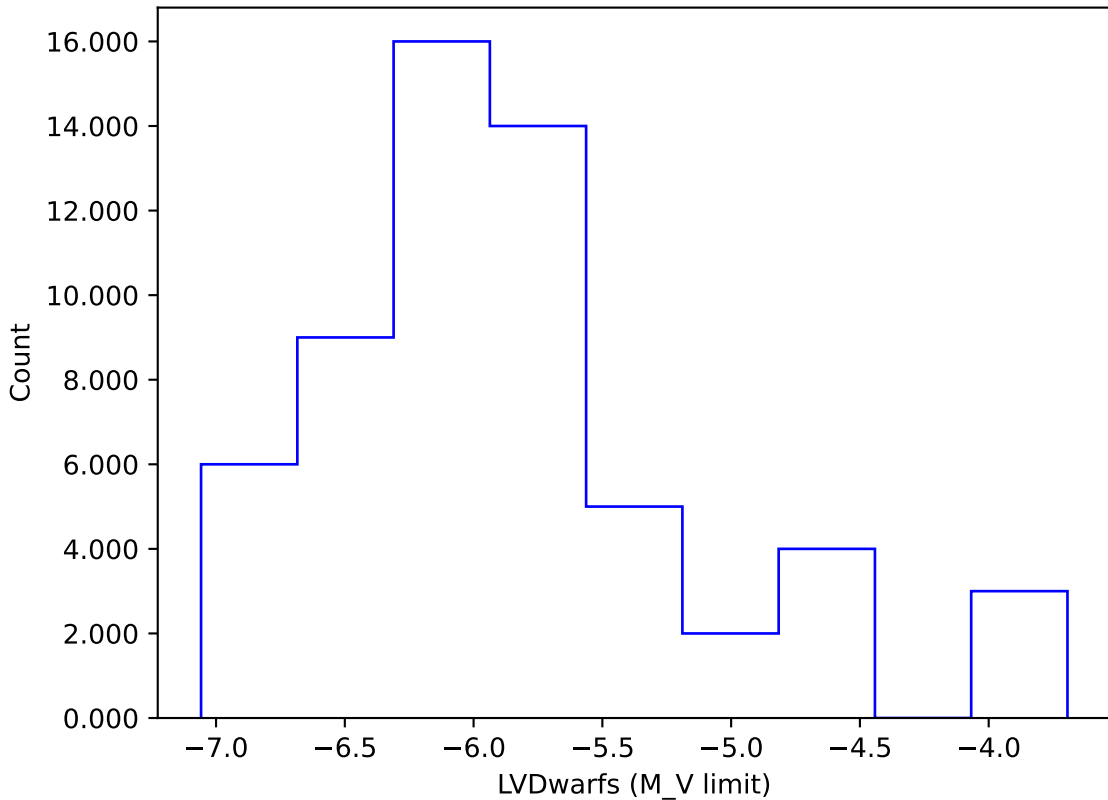
weather_cloudso12v3.5_10yrs gi: LVDwarfs
