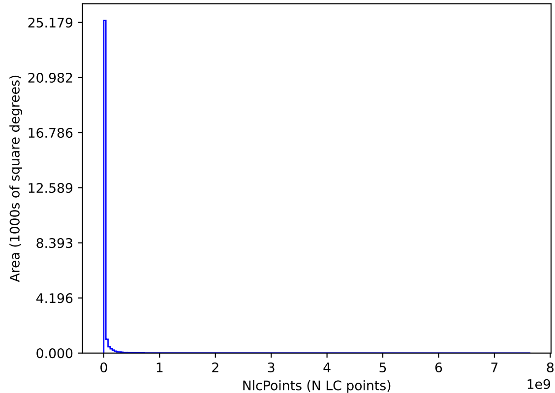
weather_cloudso12v3.5_10yrs : NlcPoints
