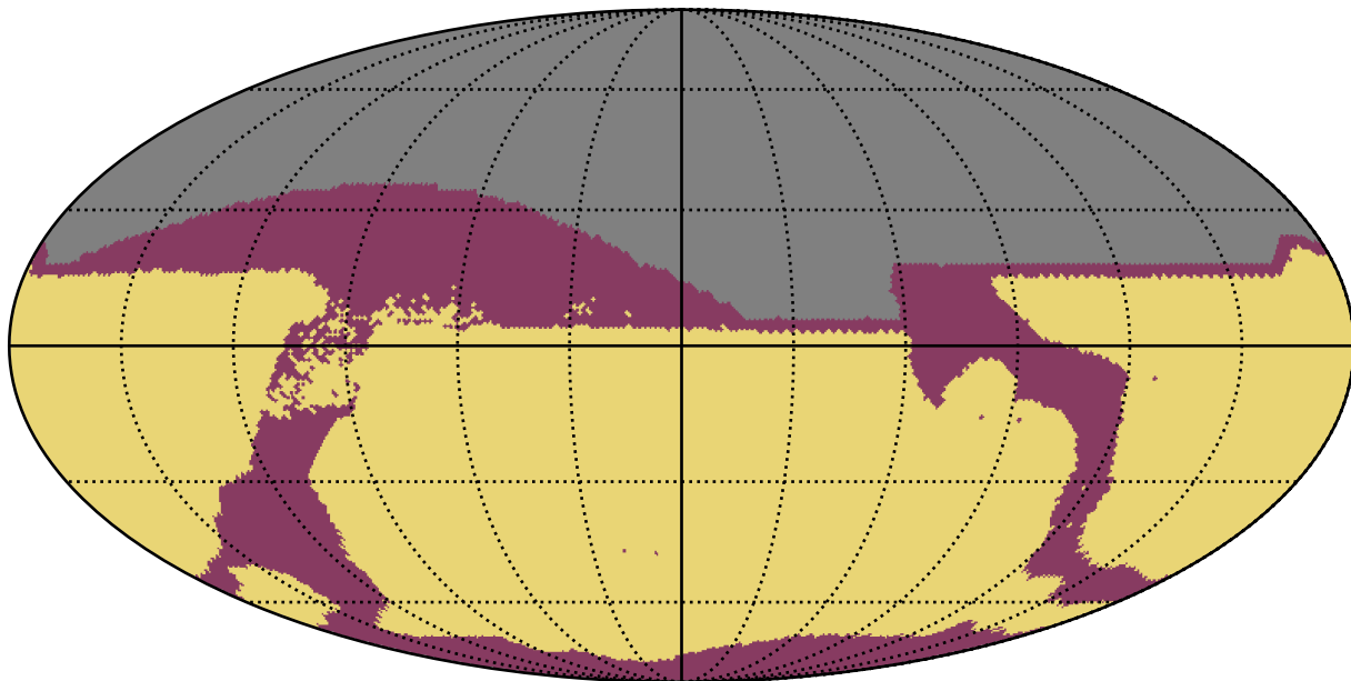
weather_cloudso12v3.5_10yrs : RapidRevisits
