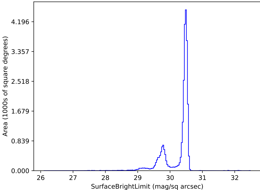
weather_cloudso12v3.5_10yrs r: SurfaceBrightLimit
