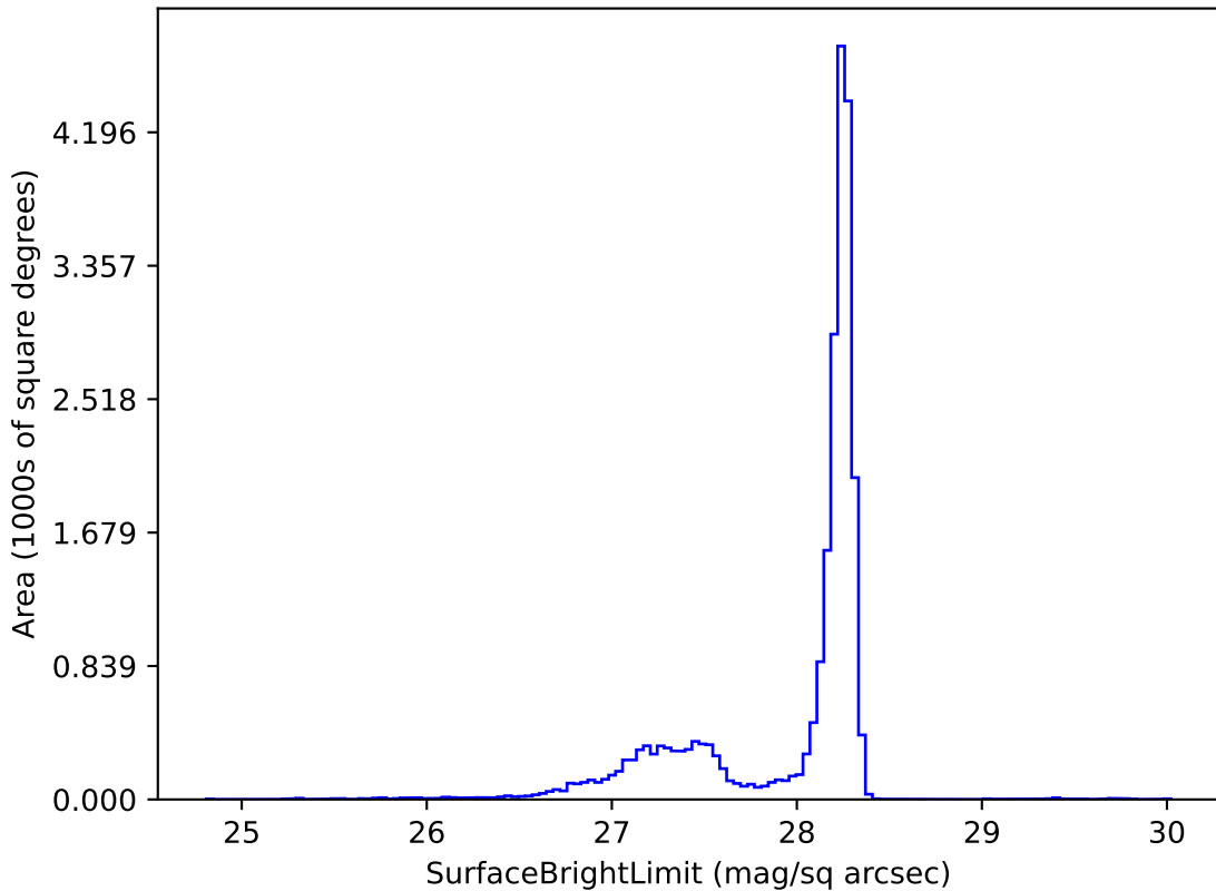
weather_cloudso12v3.5_10yrs y: SurfaceBrightLimit
