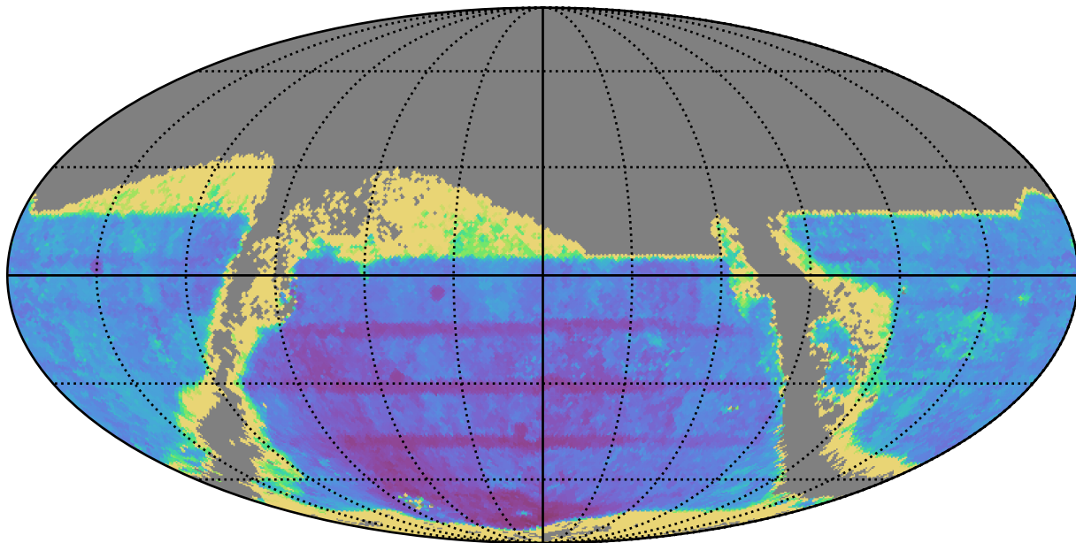
weather_cloudso12v3.5_10yrs : TDC_accuracy
