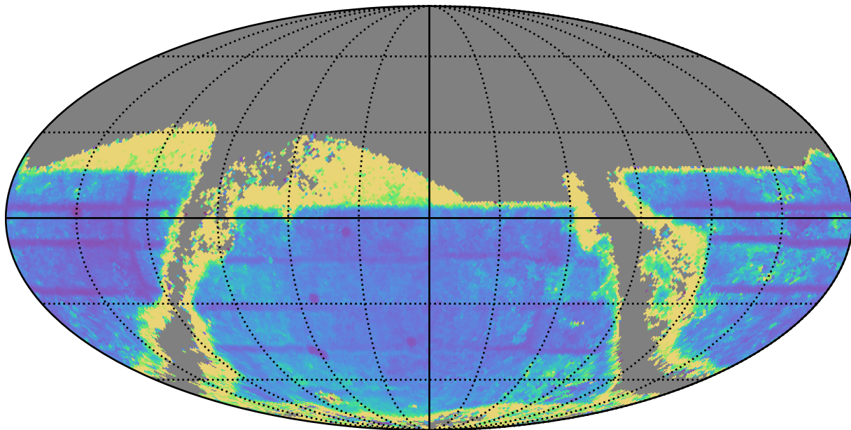
weather_cloudso12v3.5_10yrs : TDC_cadence
