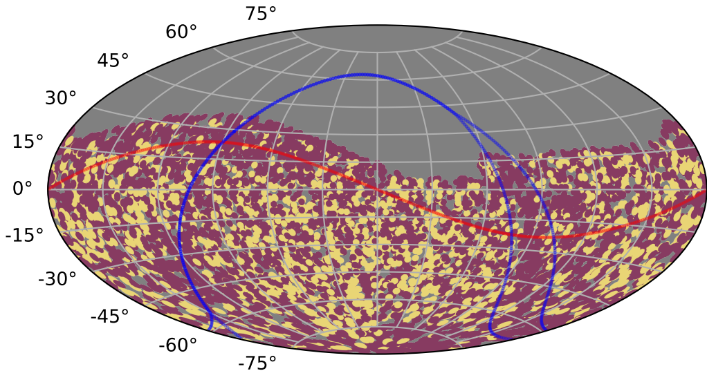
weather_cloudso12v3.5_10yrs : TDEsPopMetric_prepeak
