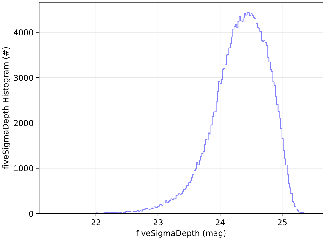
weather_cloudso12v3.5_10yrs g: fiveSigmaDepth Histogram
