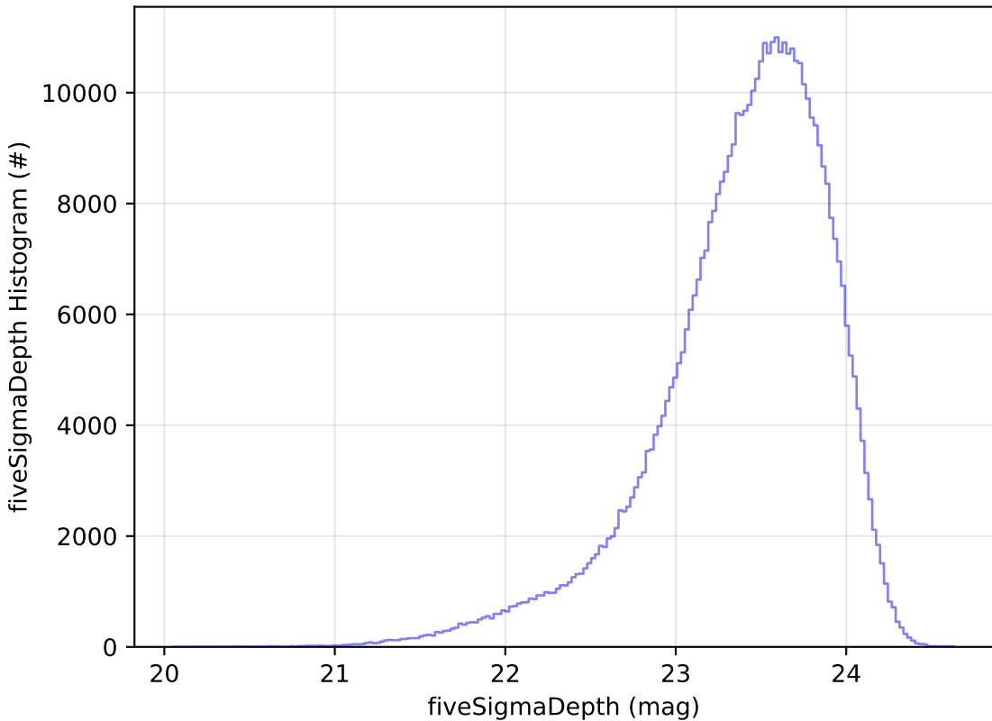
weather_cloudso12v3.5_10yrs i: fiveSigmaDepth Histogram
