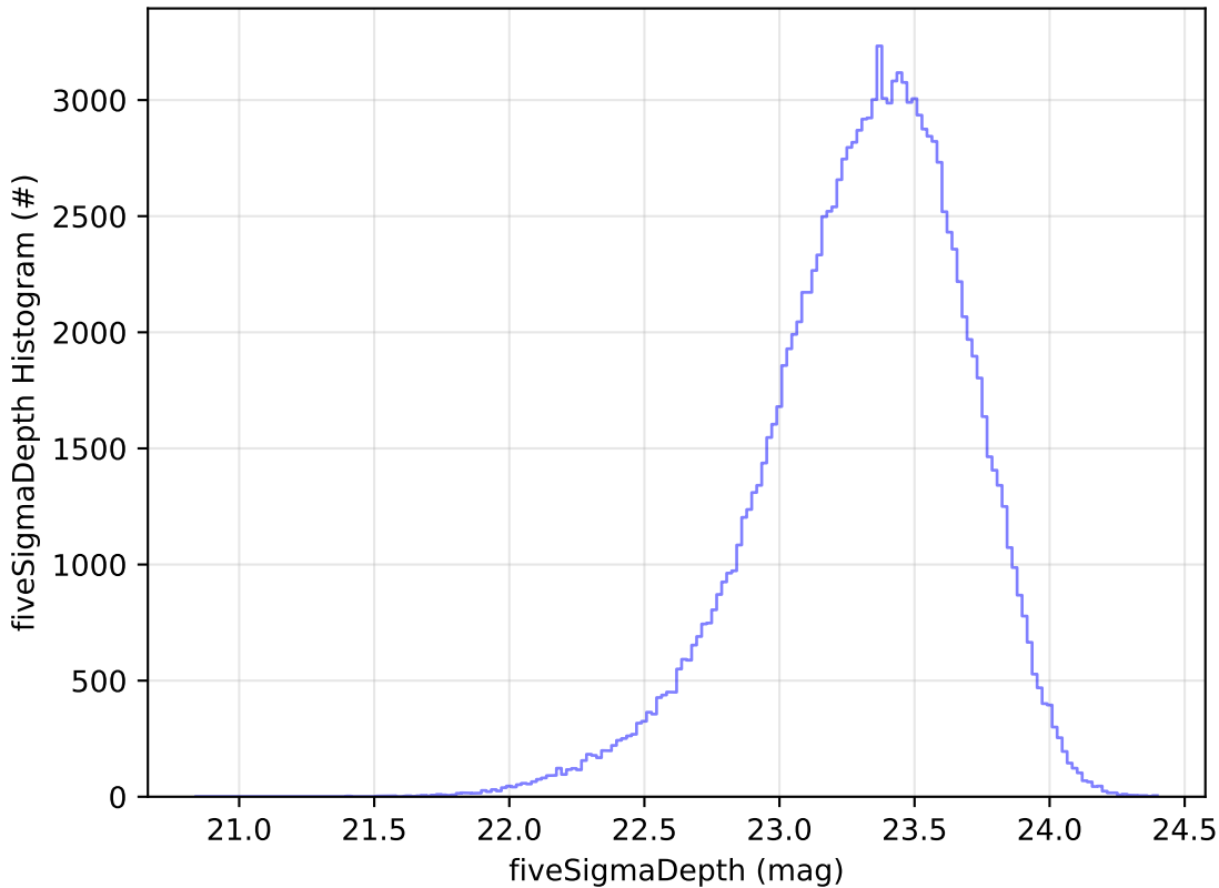
weather_cloudso12v3.5_10yrs u: fiveSigmaDepth Histogram
