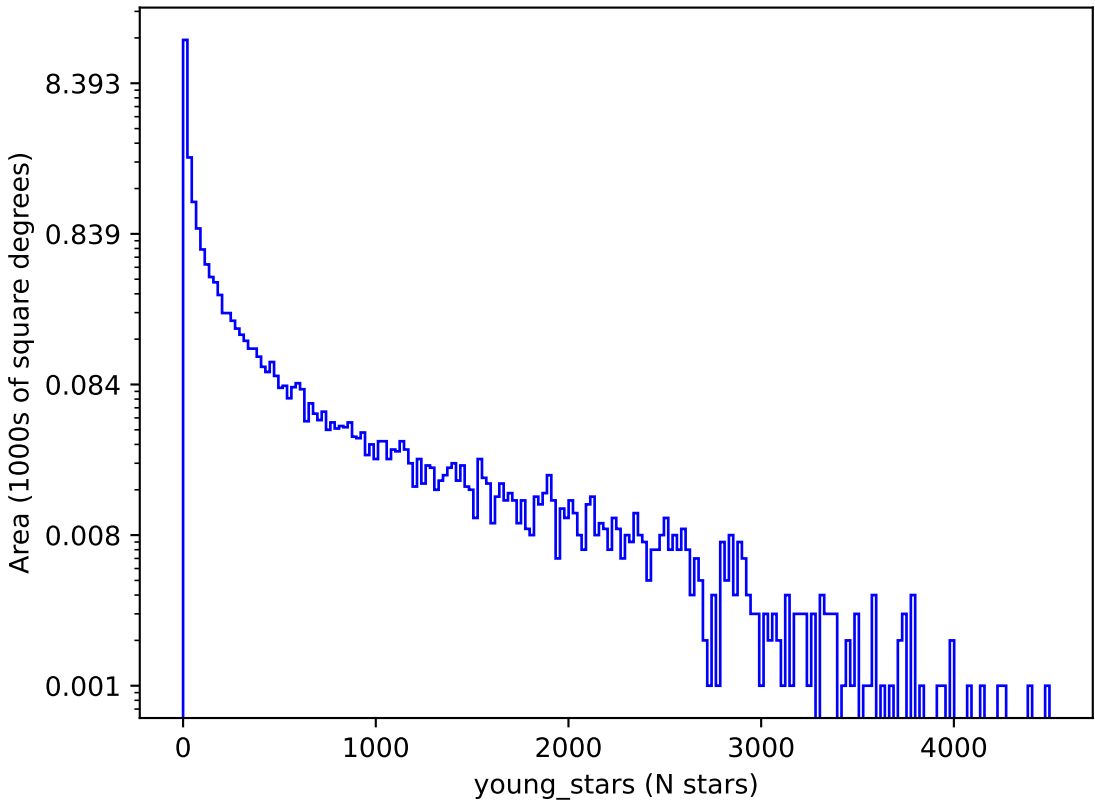
weather_cloudso12v3.5_10yrs : young_stars
