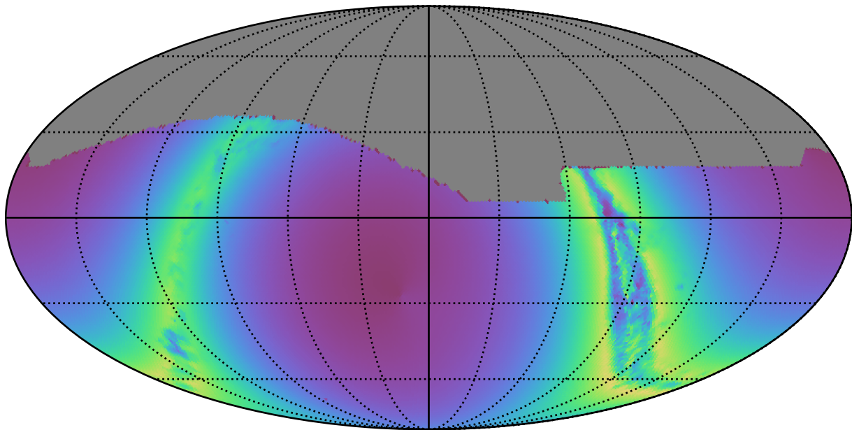
weather_cloudso12v3.5_10yrs : young_stars
