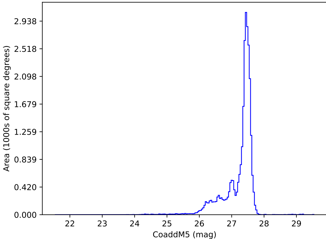
weather_cloudso14v3.5_10yrs : CoaddM5
