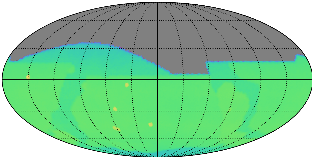
weather_cloudso14v3.5_10yrs : CoaddM5
