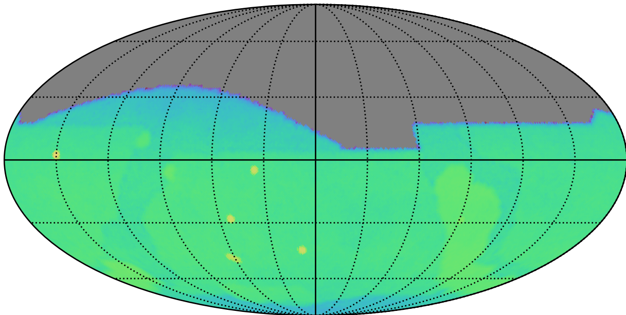
weather_cloudso14v3.5_10yrs g: CoaddM5
