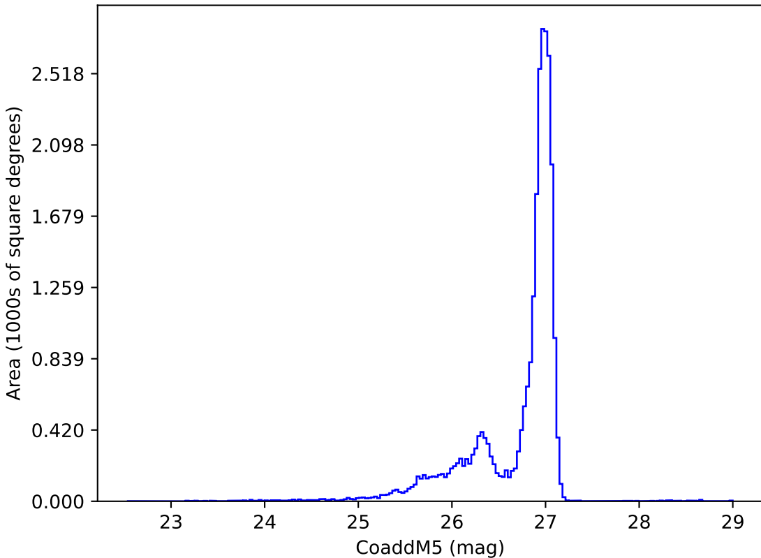
weather_cloudso14v3.5_10yrs r: CoaddM5
