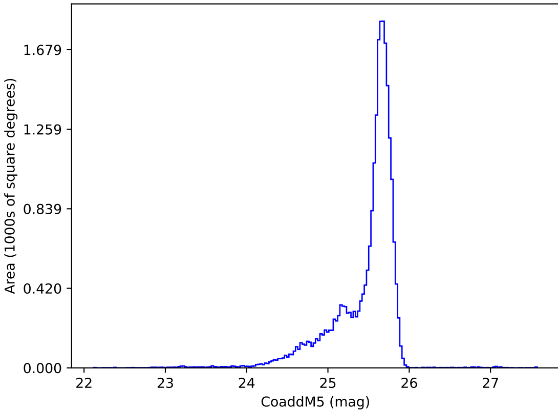
weather_cloudso14v3.5_10yrs u: CoaddM5
